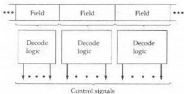
(a) Direct encoding
