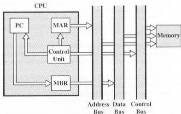
Figure 12.8 Data Flow, Interrupt Cycle
