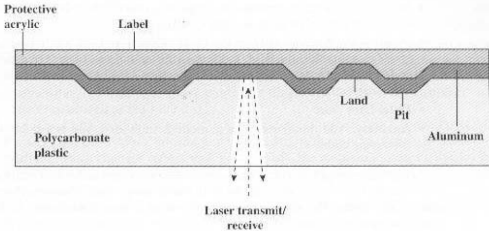
Figure 6.10 CD Operation
