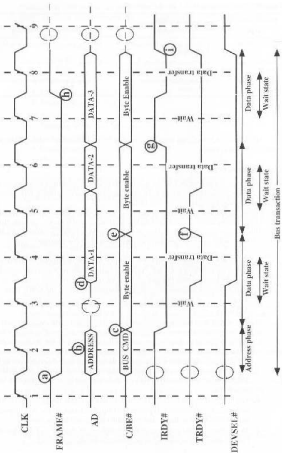
Figure 3.23 PCI Read Operation
