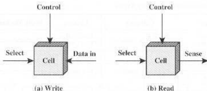
Figure 5.1 Memory Cell Operation
