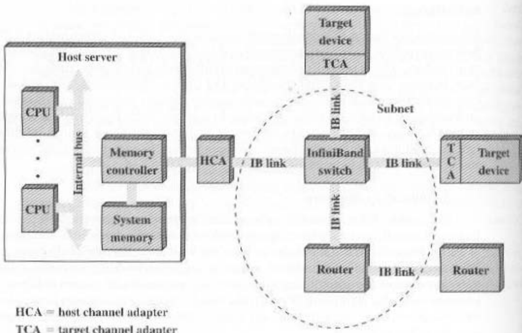
Figure 7.20 InfiniBand Switch Fabric
