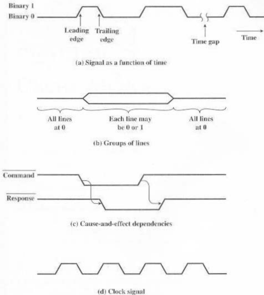
Figure 3.27 Timing Diagrams
