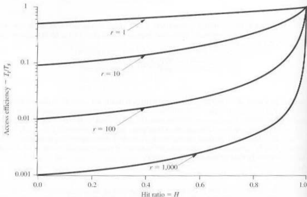
Figure 4.19 Access Efficiency as a Function of hit Ratio ( r = T_2/T_s )
