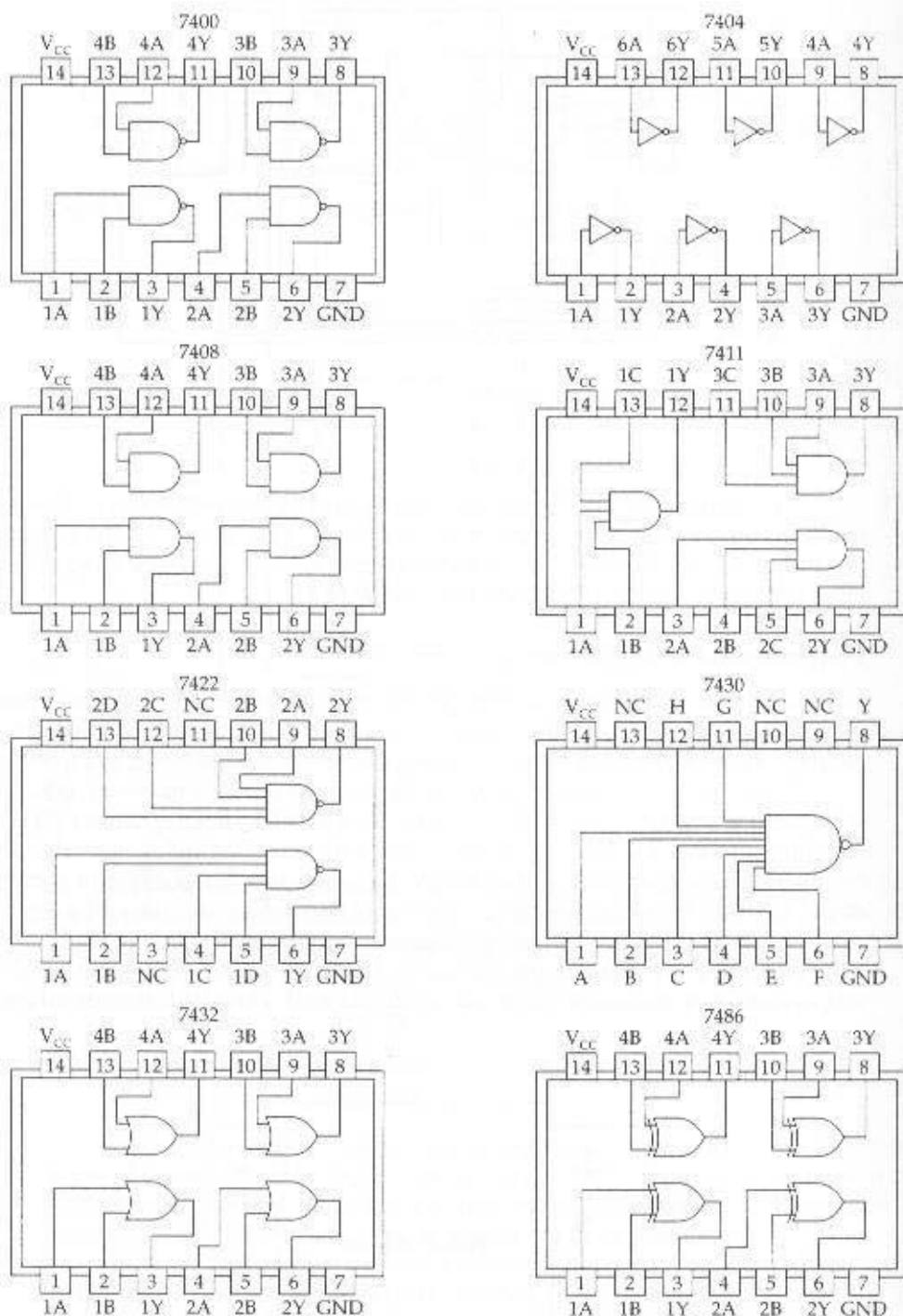
Figure A.18 Some SSI Chips. Pin layouts from The TTL Data Book for Design Engineers , copyright © 1976 Texas Instrument Incorporated.
