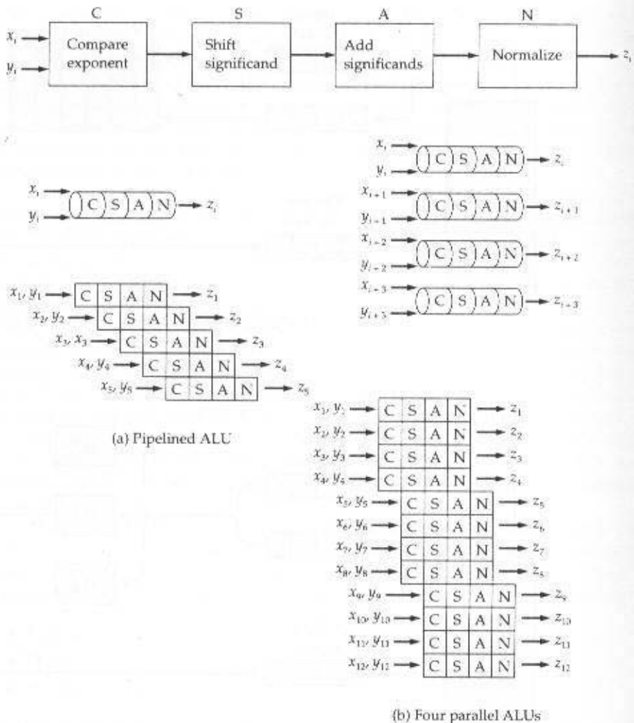
Figure 18.15 Pipelined Processing
