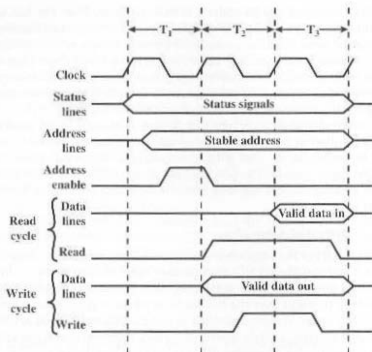
Figure 3.19 Timing of Synchronous Bus Operations
