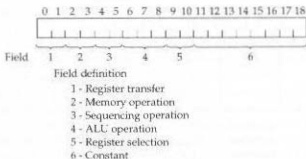
(b) Horizontal microinstruction format
