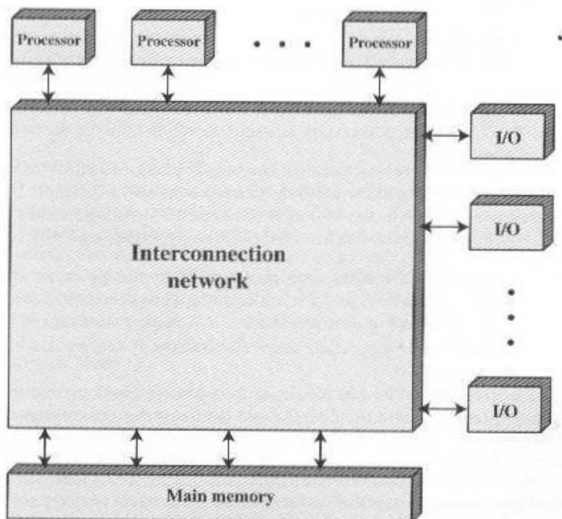
Figure 18.4 Generic Block Diagram of a Tightly Coupled Multiprocessor
