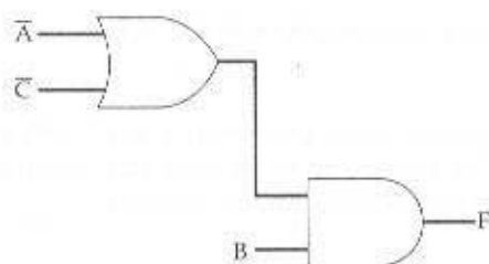
Figure A.6 Simplified Implementation of Table A.3
