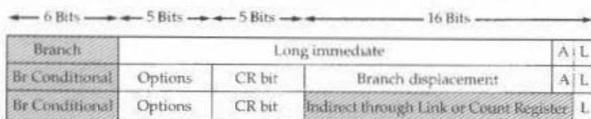
(a) Branch instructions
