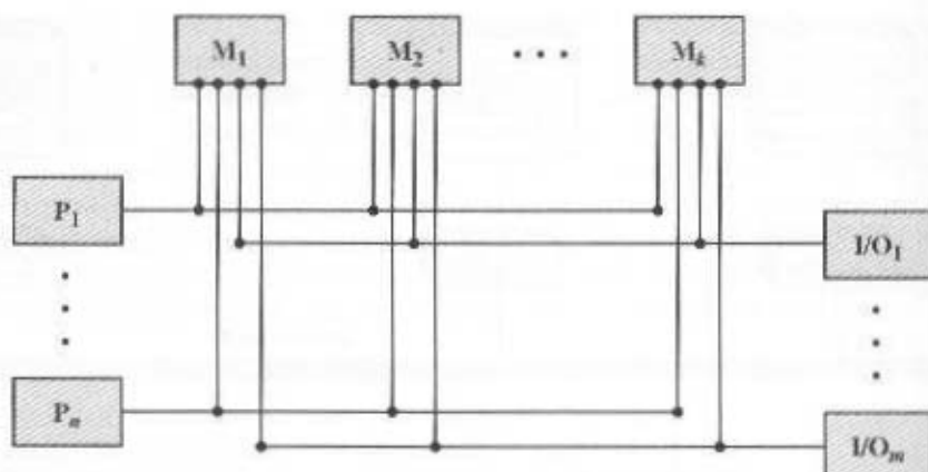
Figure 18.6 Multiport Memory
