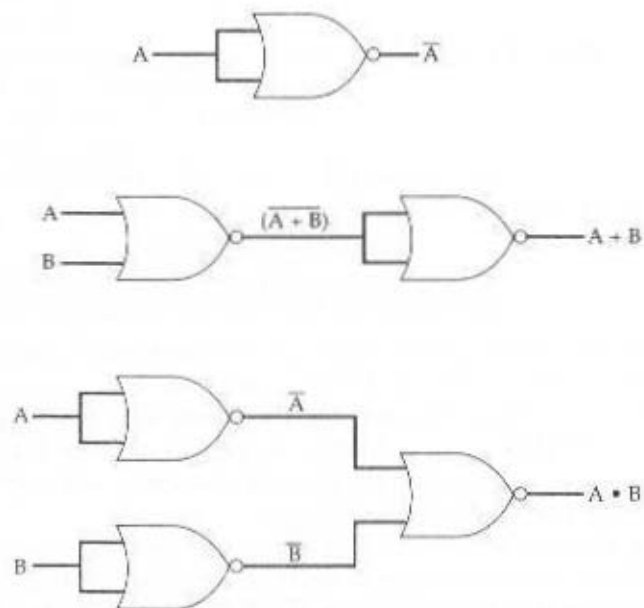
Figure A.3 The Use of NOR Gates
