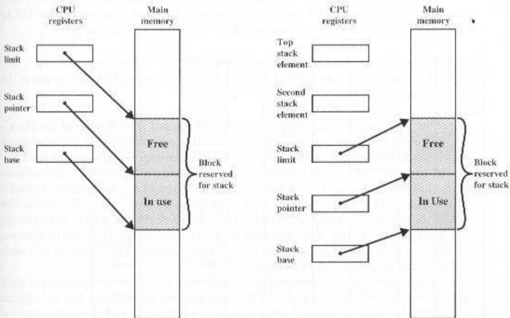
(a) All of stack in memory
