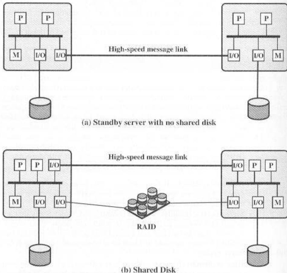
Figure 18.9 Cluster Configurations
