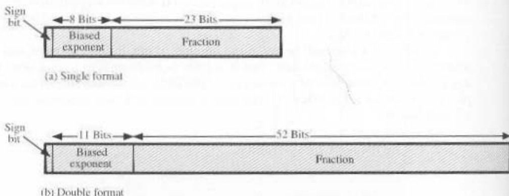
Figure 9.21 IEEE 754 Formats
