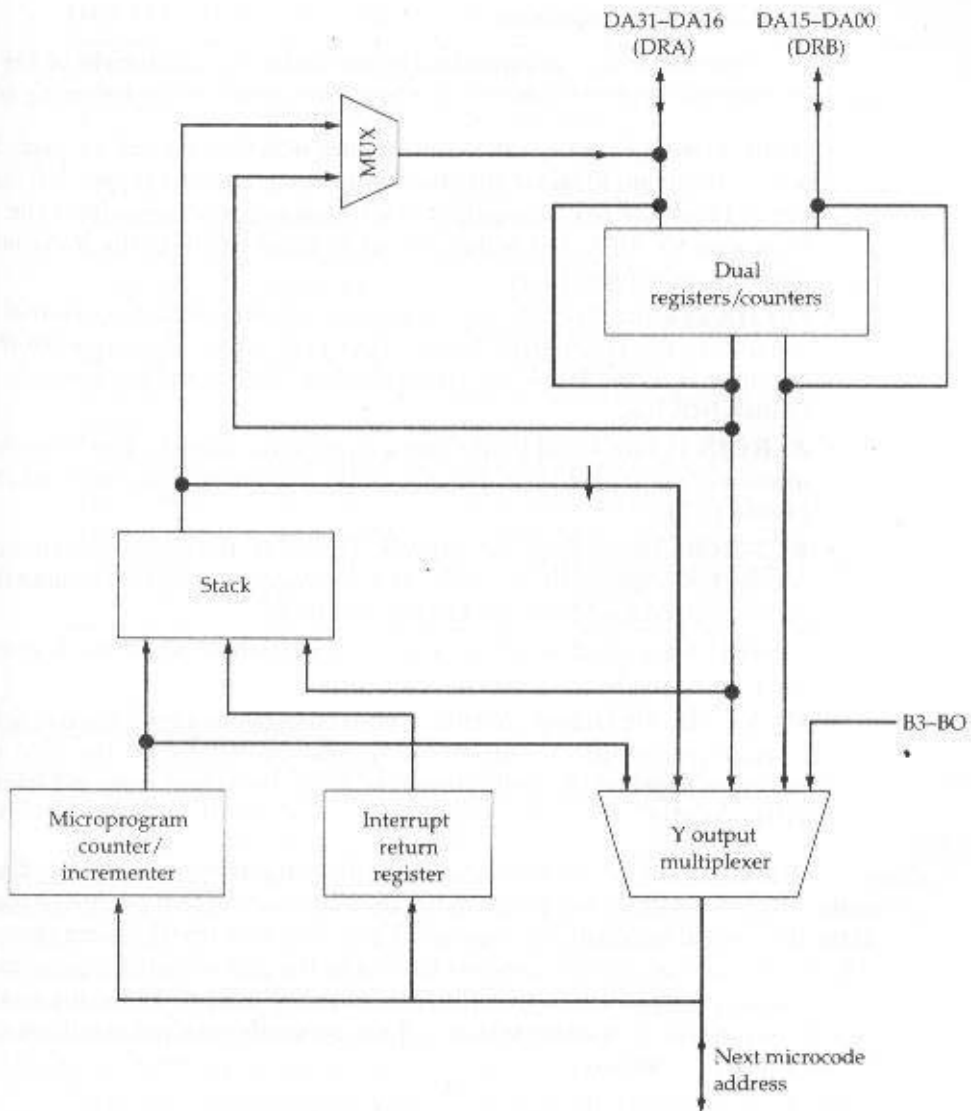
Figure 17.18 TI 8818 Microsequencer
