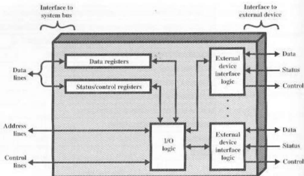
Figure 7.4 Block Diagram of an I/O Module
