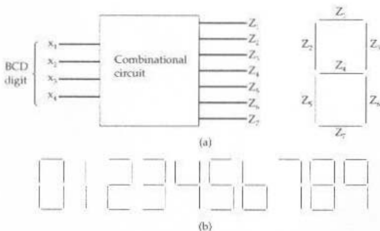
Figure A.34 Seven-Segment LED Display Example
