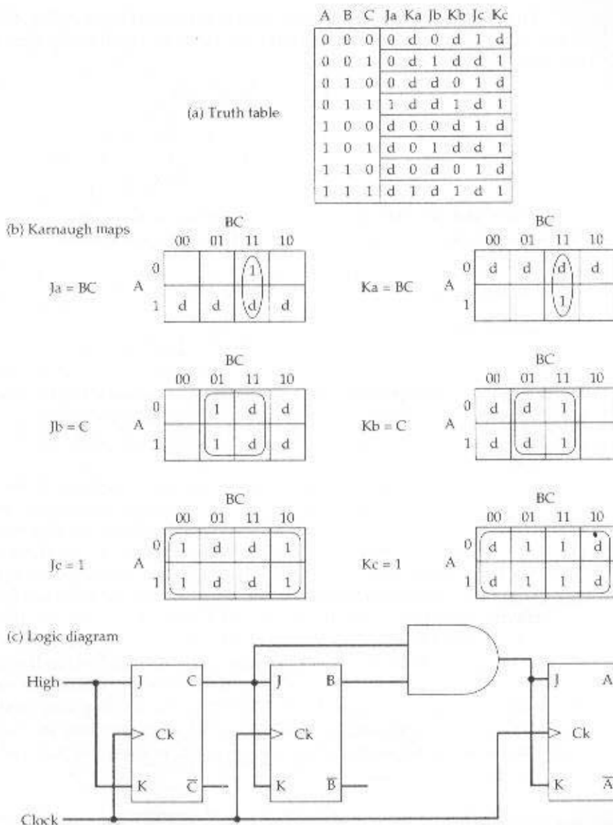
Figure A.33 Design of a Synchronous Counter
