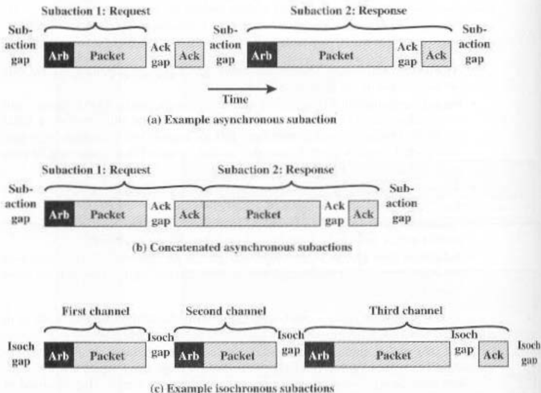
Figure 7.19 FireWire Subactions
